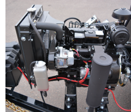
Motor diesel
